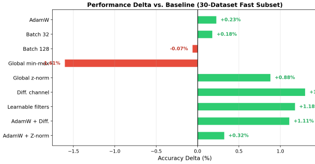
Fig. 2. Mean accuracy comparison across different configurations. Batch size 32 achieved slightly higher accuracy than the baseline, while batch size 128 resulted in a small accuracy reduction.
